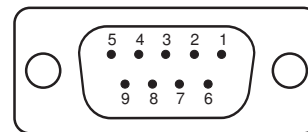
Pin side view of female DB9
