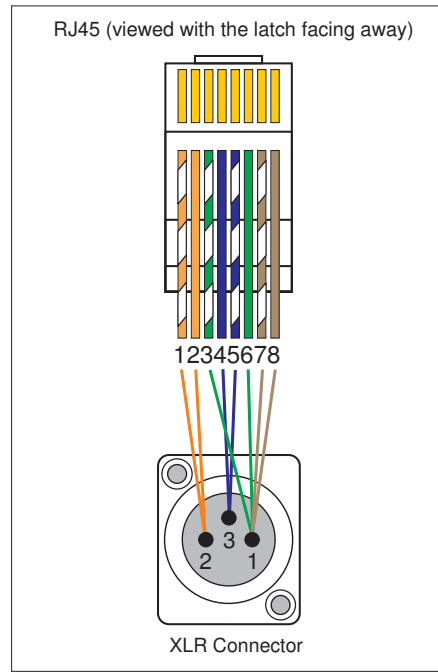
Suggested CAT5 adaptor wiring
