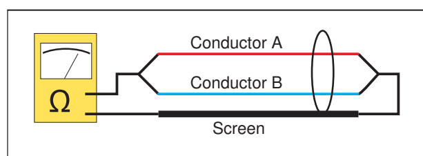
Measuring DC Loop resistance.
